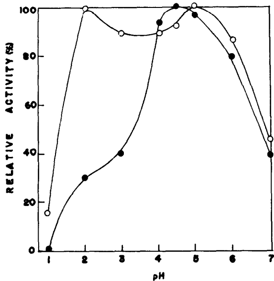
Fig. 1. Activity-pH relation curve of fucoidanase in comparison with that of α-L-fucosidase. pH 1.0 to 2.0, 0.017 M citrate-HCl buffer; pH 3.0 to 7.0, 0.017 M citrate-0.034 M phosphate buffer. ●—●, Fucoidanase; ○—○, α-L-fucosidase.
