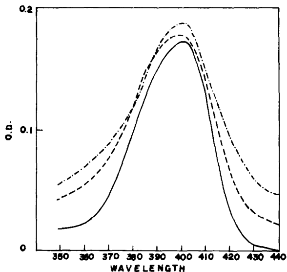
Fig. 4. Comparison of absorption spectra of chromogens produced by reaction with cysteine-sulfuric acid (5). - - - - -, The sugar product showing R_f 0.43; - · - · - ·, the sugar product showing R_f 0.34; —, L-fucose (see fig. 3).
